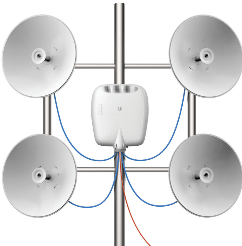
Example of a Backhaul Deployment for the EdgePoint
