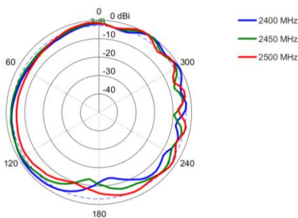
Azimuth: 2400 – 2500 MHz
