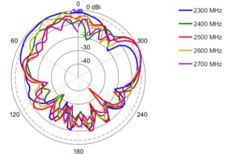
Elevation 1: 2300 – 2700 MHz
