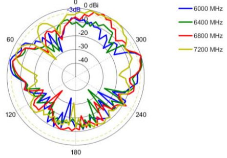
Elevation: 6000 – 7200 MHz
