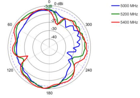
Azimuth: 5000 – 5400 MHz
