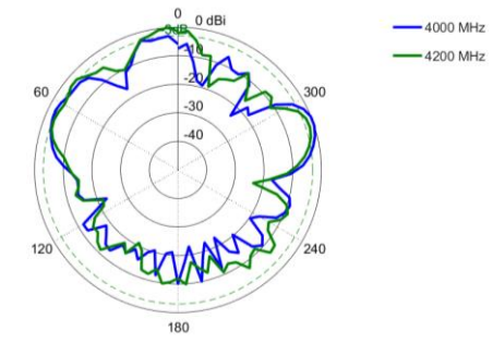
Elevation 2: 4000 – 4200 MHz
