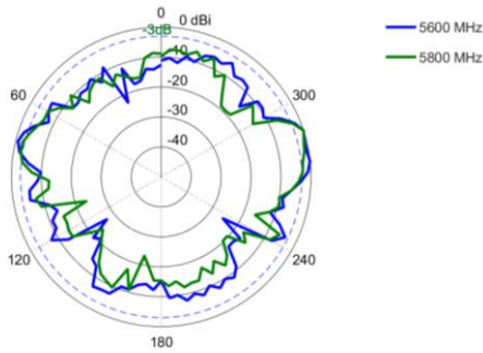
Elevation: 5600 – 5800 MHz
