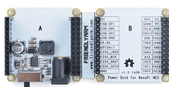
Power Dock for NanoPi NEO/Air
