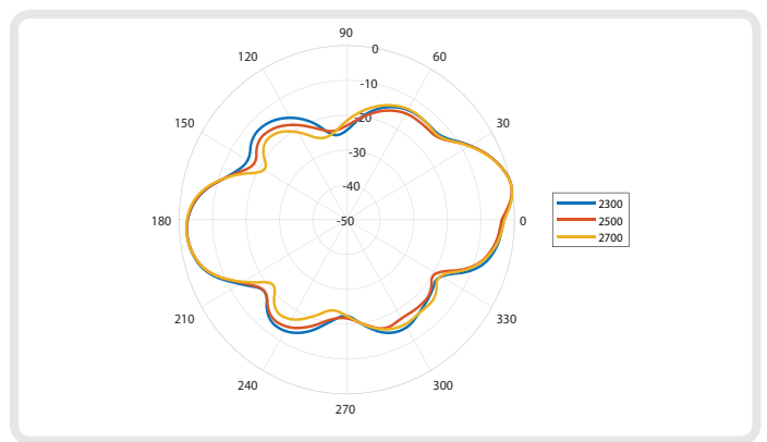
Elevation: 1700 - 2700 MHz
