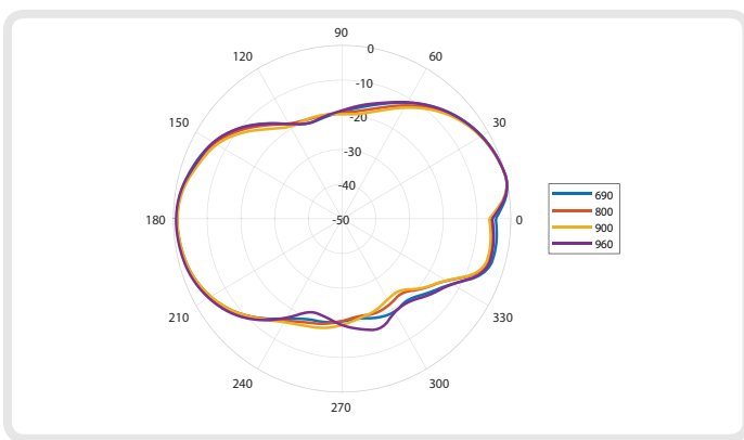
Elevation: 690 - 960 MHz
