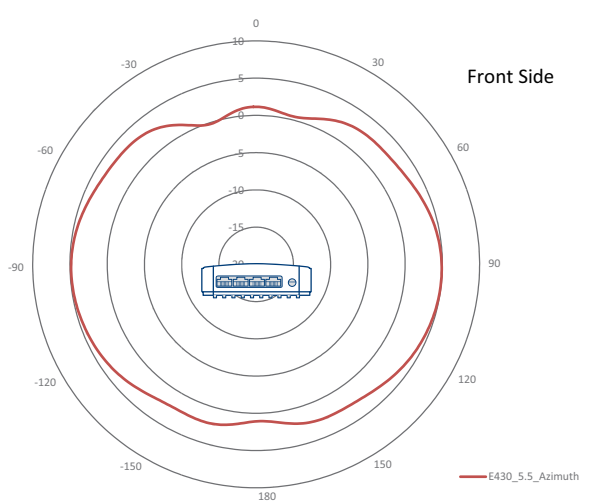
5 GHz Azimuth
