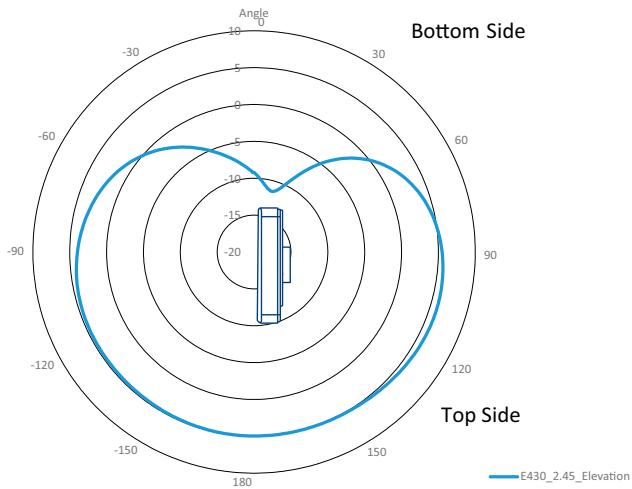
2.4 GHz Elevation
