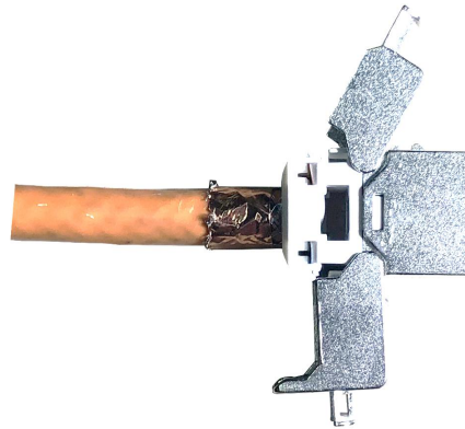
⑧.install the temination cap in direction of arrow into the keystone jack
