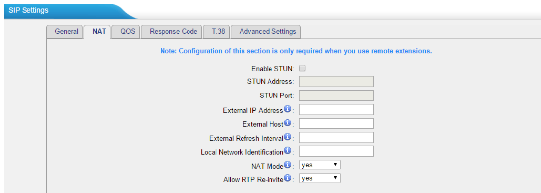
Figure 5-5 NAT Settings
