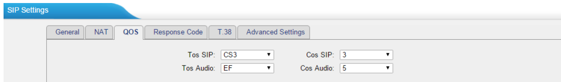
Figure 5-6 Qos
