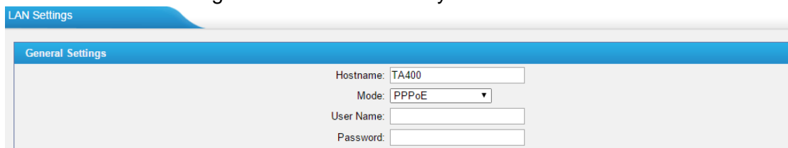
Figure 9-3 PPPoE
