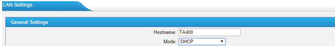
Figure 9-2 DHCP Mode
