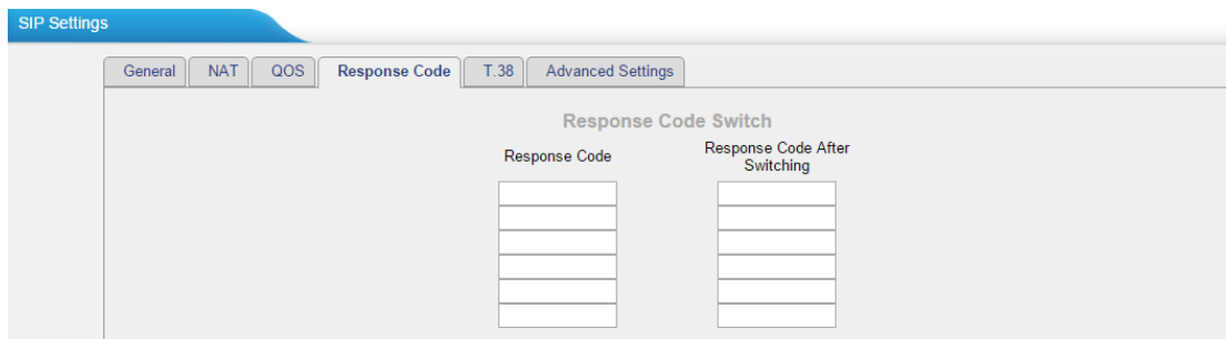
Figure 5-7 Response Code
